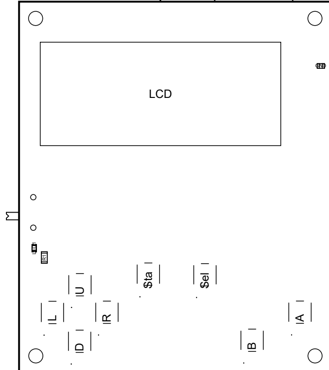
View from Top side (Scale 1:1)
