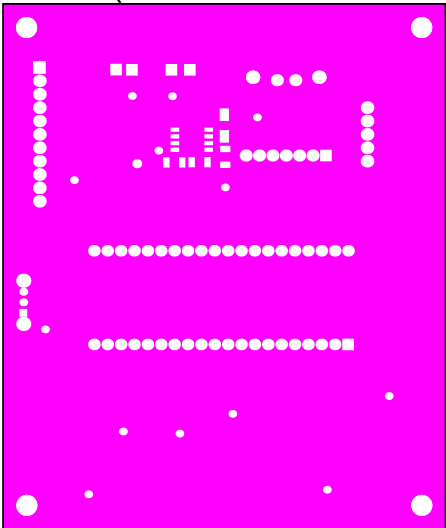
Bottom Solder (Scale 1:1.43533802210421)
