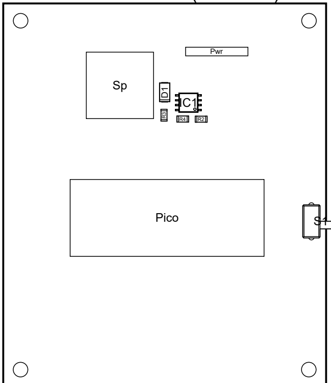
View from Bottom side (Scale 1:1)
