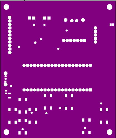
Top Solder (Scale 1:1.40904607580668)
